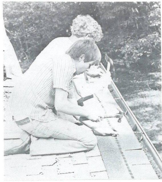
Workshops unite our schools, not only in labor but in spirit as we prepare for service.
