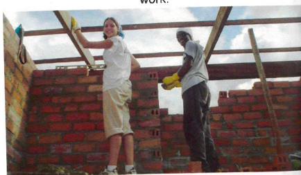
Honiko and Vyn try to finish laying blocks so other team members can start putting the roof on.
